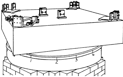
FIG. 2. The Michelson-Morley interferometer of 1887.
