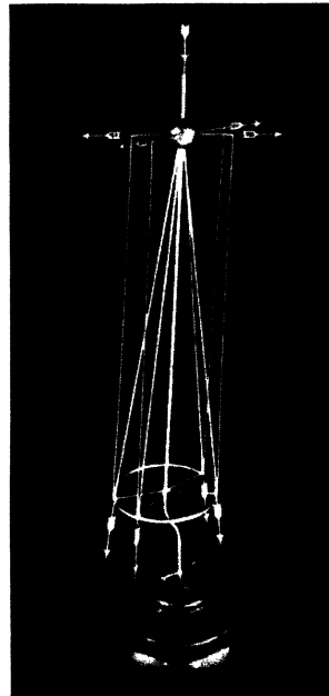
FIG. 29. Model illustrating the components of ether-drift.
