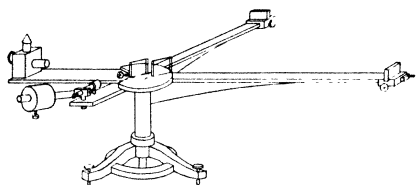
FIG. 1. Michelson's ether-drift interferometer of 1881.
